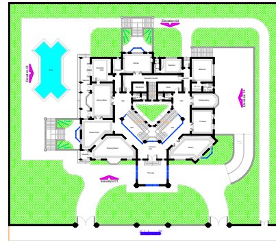
First Floor Plan A = 567,71 m 2
