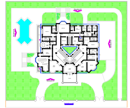
Second Floor Plan A = 493,92 m 2
