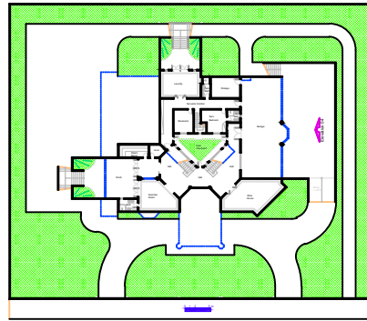
Lower Floor Plan A = 423,28 m 2
